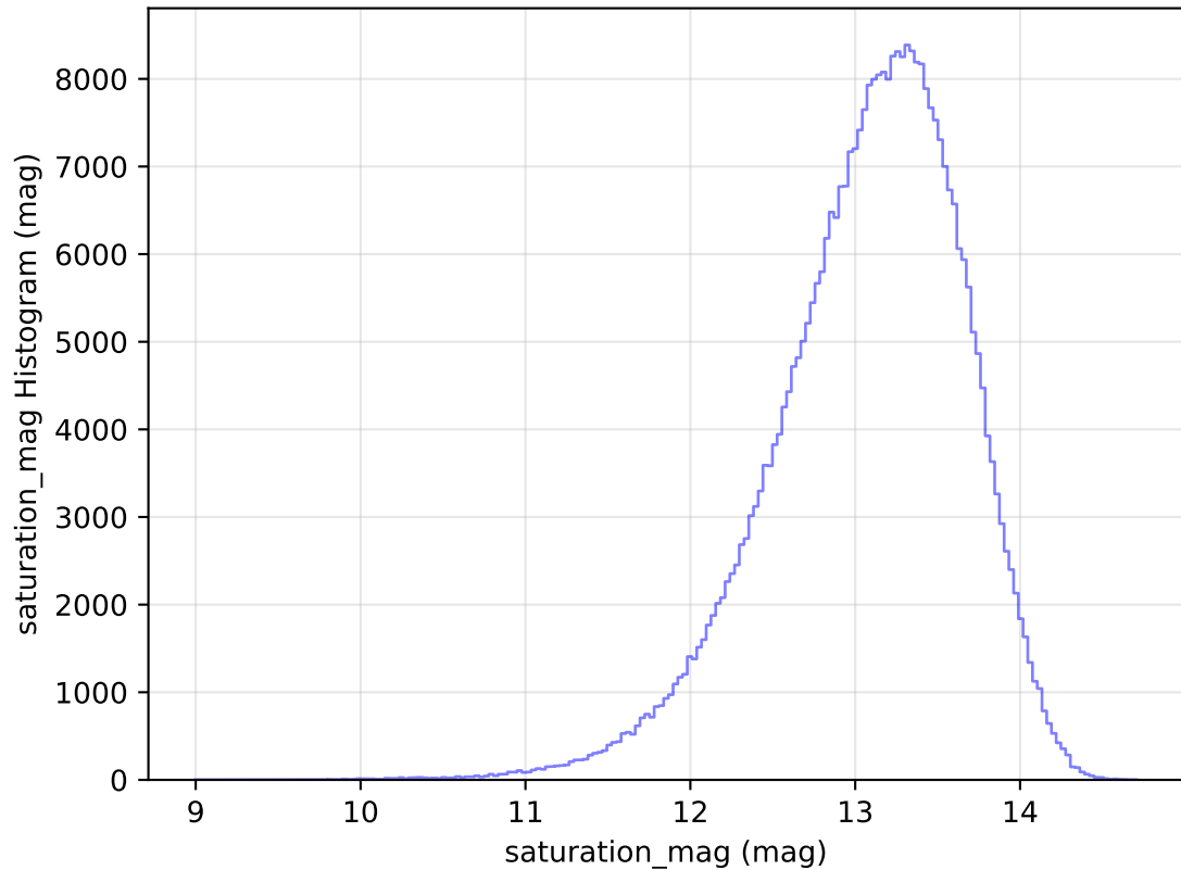
too_elab_heavy_r128_d2_ugrizy_v3.4_10yrs WFD y band: saturation_mag Histogram
