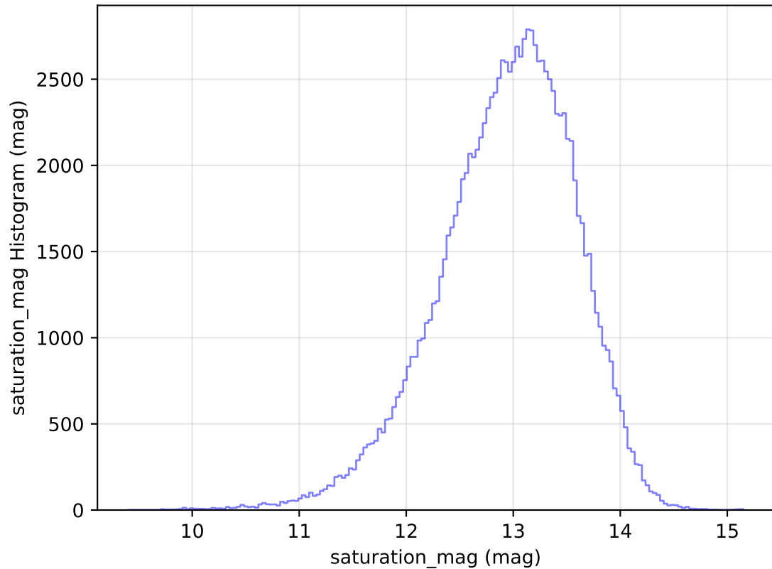
too_elab_heavy_r128_d2_ugrizy_v3.4_10yrs WFD u band: saturation_mag Histogram
