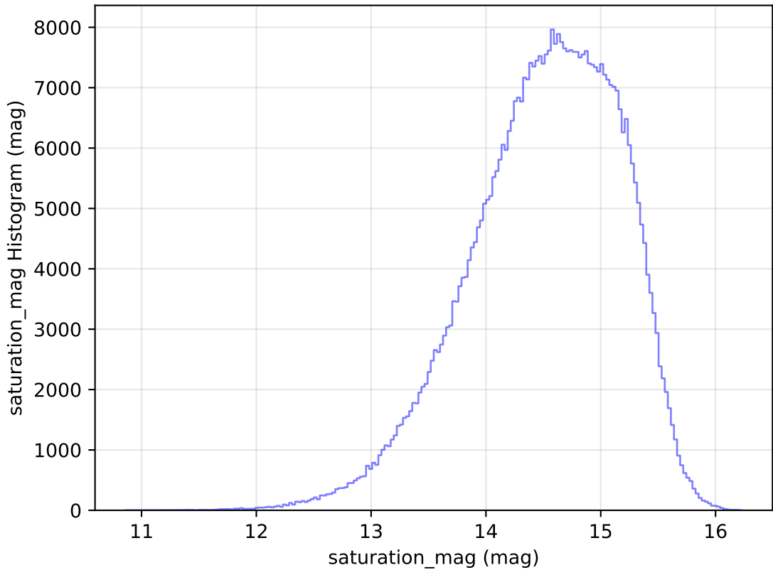
too_elab_heavy_r128_d2_ugrizy_v3.4_10yrs WFD r band: saturation_mag Histogram
