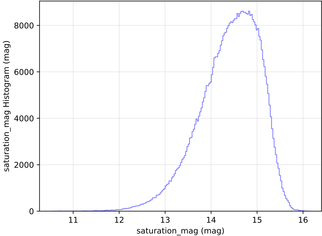
too_elab_heavy_r128_d2_ugrizy_v3.4_10yrs WFD i band: saturation_mag Histogram
