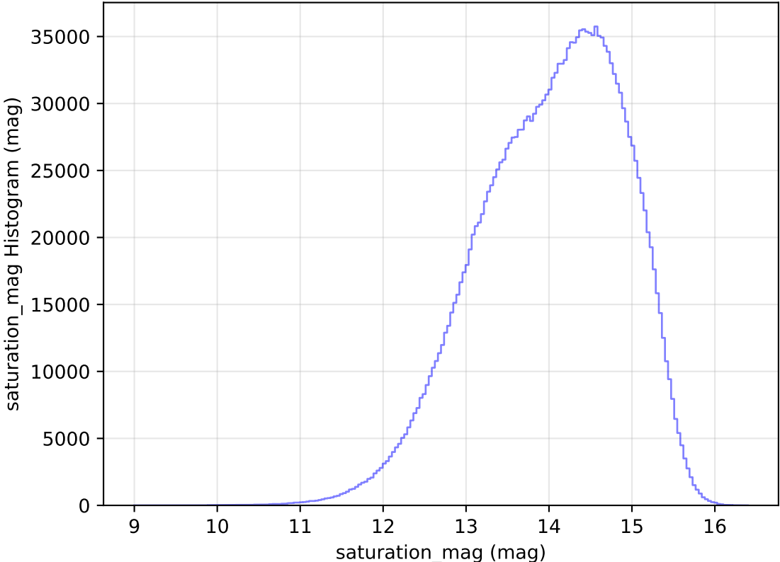
too_elab_heavy_r128_d2_ugrizy_v3.4_10yrs WFD all bands: saturation_mag Histogram
