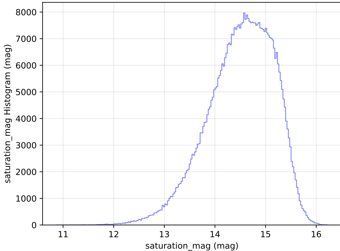
too_elab_heavy_r128_d2_ugrizy_v3.4_10yrs All sky r band: saturation_mag Histogram
