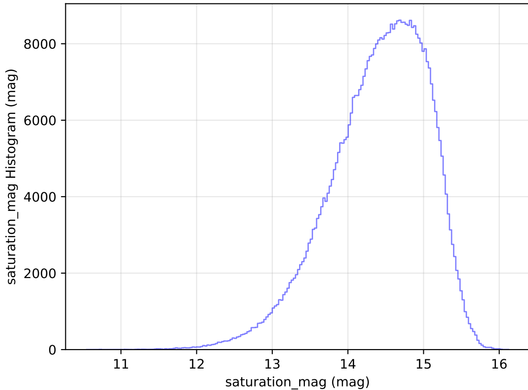
too_elab_heavy_r128_d2_ugrizy_v3.4_10yrs All sky i band: saturation_mag Histogram
