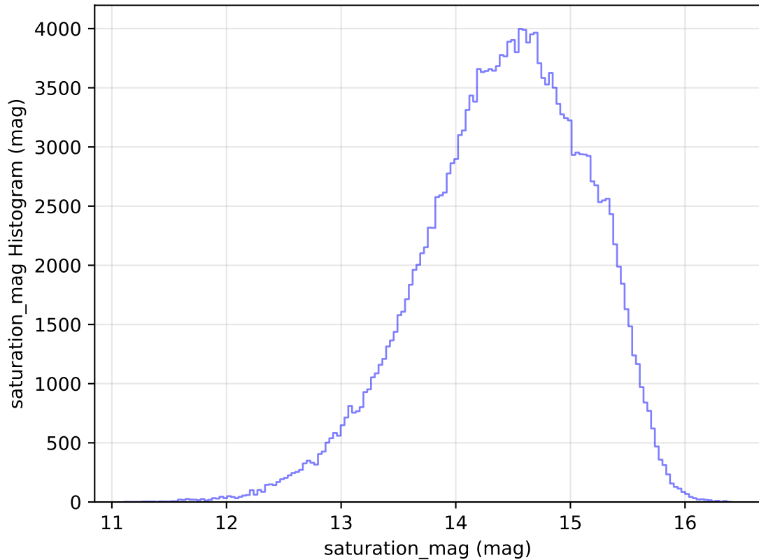
too_elab_heavy_r128_d2_ugrizy_v3.4_10yrs All sky g band: saturation_mag Histogram
