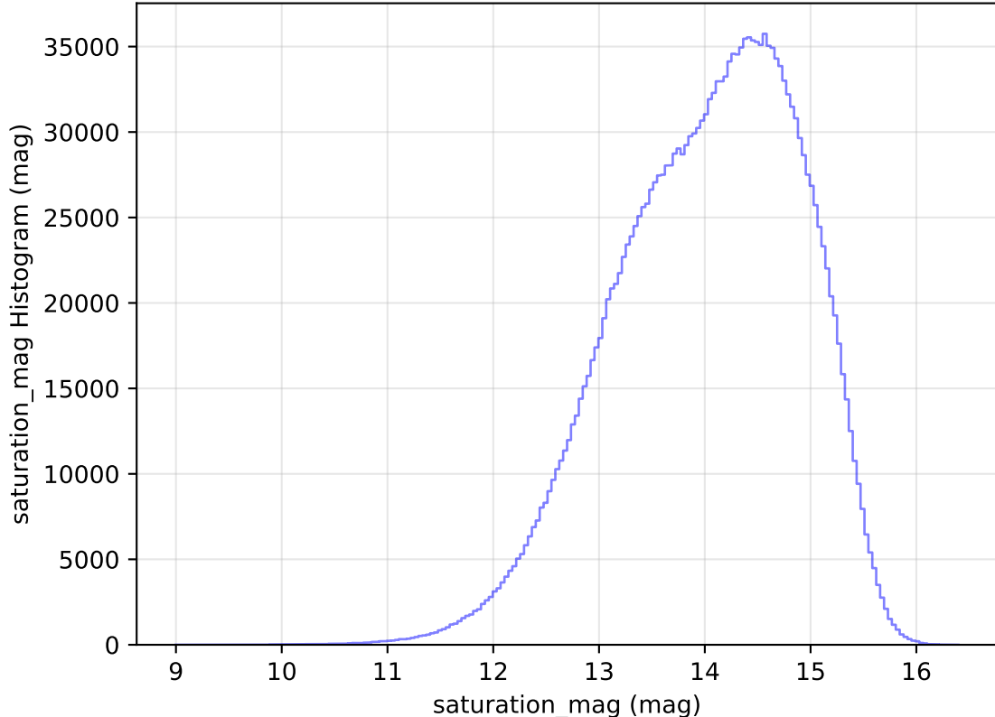
too_elab_heavy_r128_d2_ugrizy_v3.4_10yrs All sky all bands: saturation_mag Histogram
