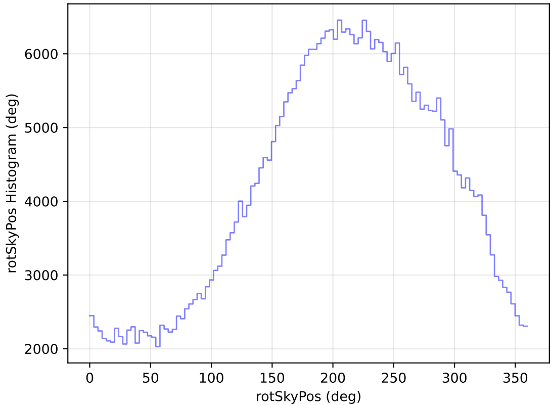
too_elab_heavy_r128_d2_ugrizy_v3.4_10yrs WFD z band: rotSkyPos Histogram
