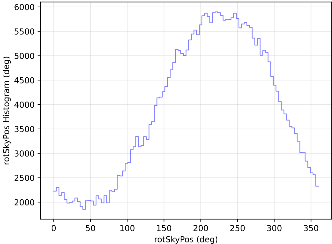
too_elab_heavy_r128_d2_ugrizy_v3.4_10yrs WFD y band: rotSkyPos Histogram
