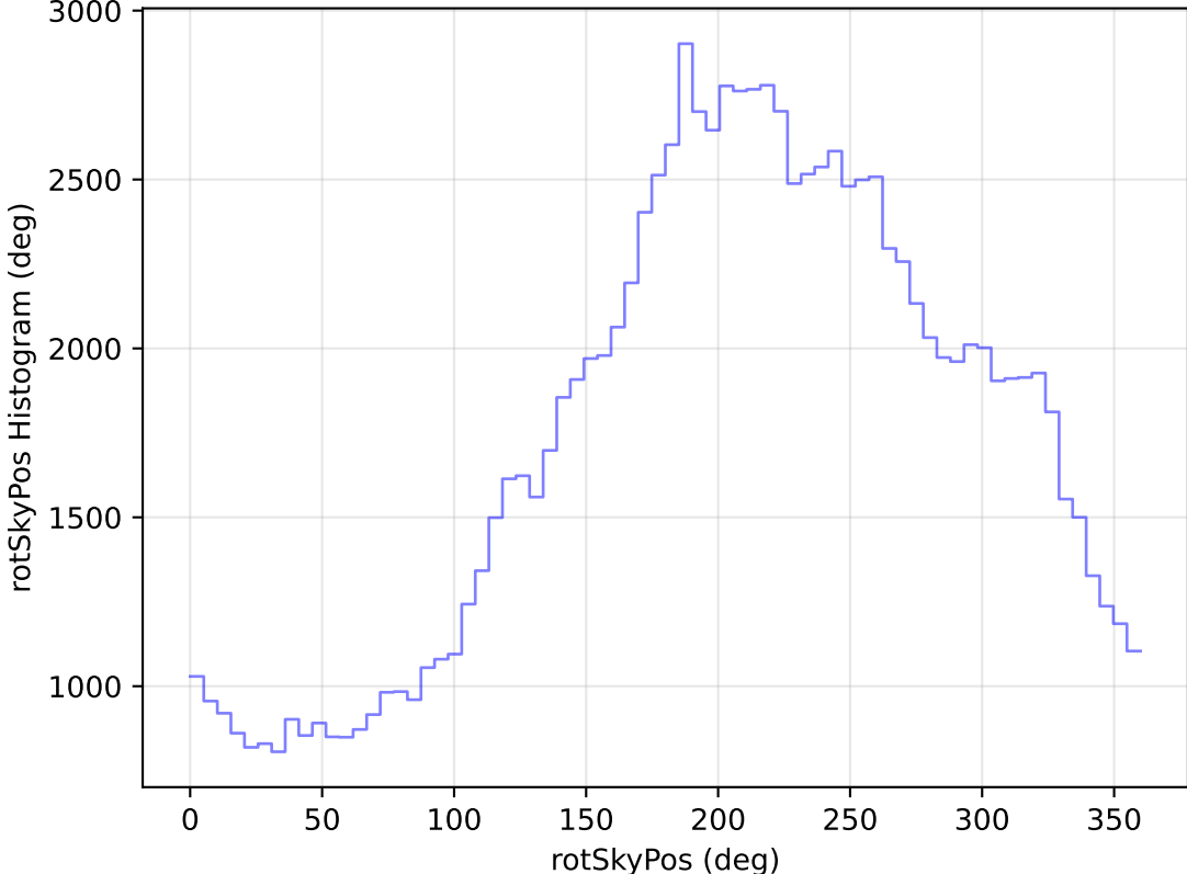
too_elab_heavy_r128_d2_ugrizy_v3.4_10yrs WFD u band: rotSkyPos Histogram
