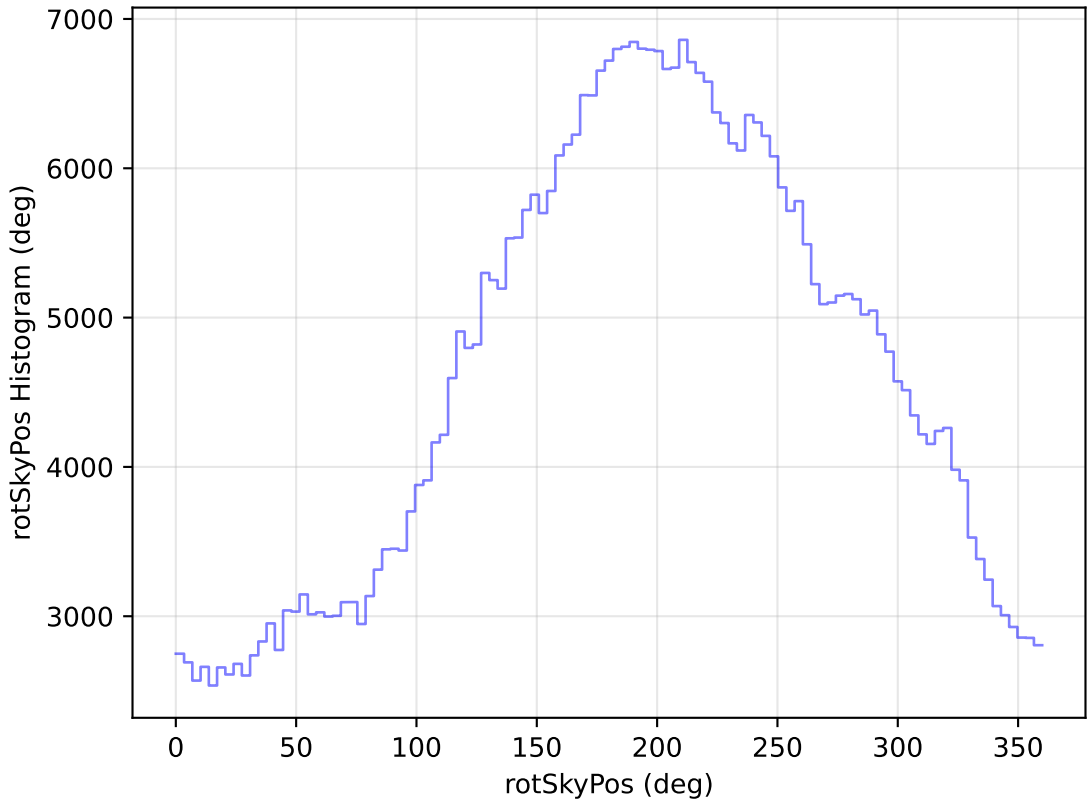
too_elab_heavy_r128_d2_ugrizy_v3.4_10yrs WFD r band: rotSkyPos Histogram
