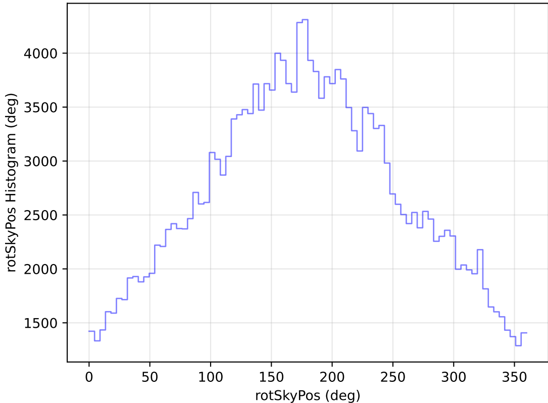
too_elab_heavy_r128_d2_ugrizy_v3.4_10yrs WFD g band: rotSkyPos Histogram
