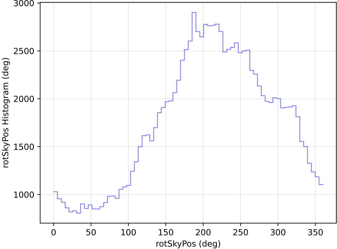
too_elab_heavy_r128_d2_ugrizy_v3.4_10yrs All sky u band: rotSkyPos Histogram
