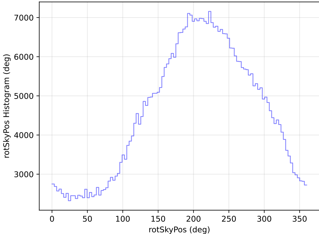
too_elab_heavy_r128_d2_ugrizy_v3.4_10yrs All sky i band: rotSkyPos Histogram
