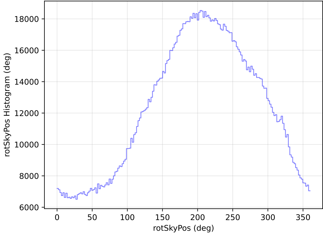
too_elab_heavy_r128_d2_ugrizy_v3.4_10yrs All sky all bands: rotSkyPos Histogram
