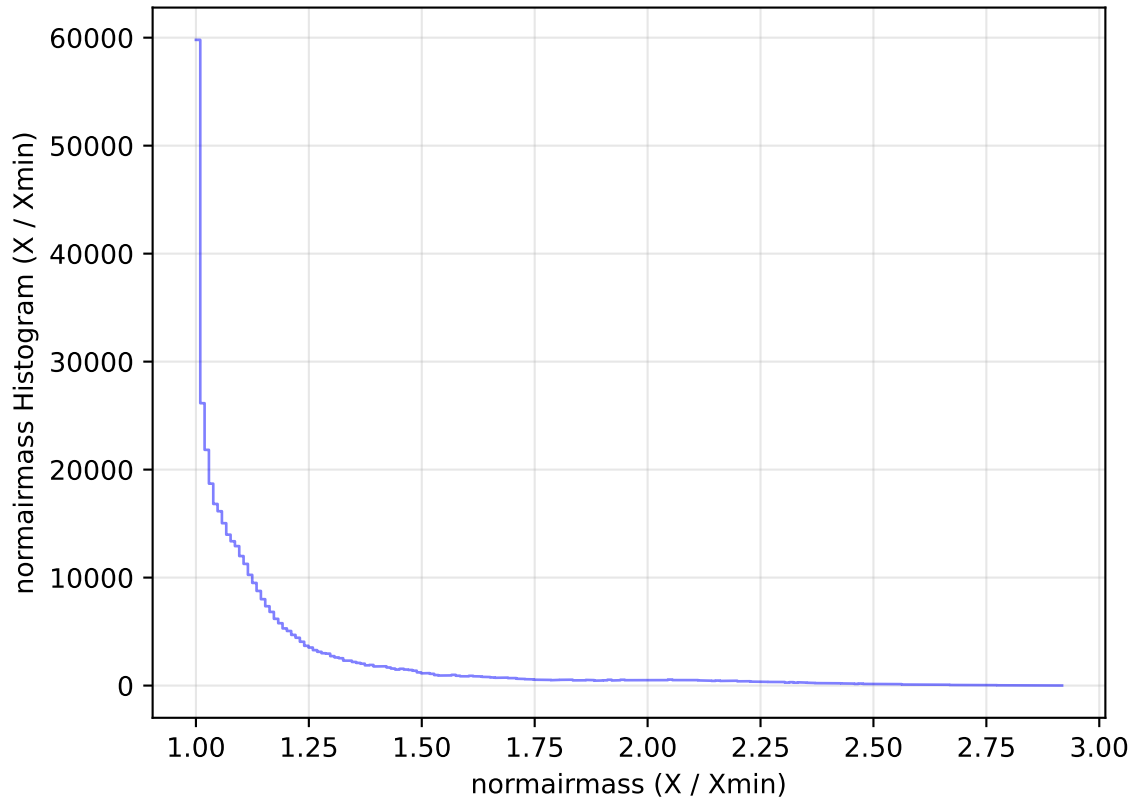
too_elab_heavy_r128_d2_ugrizy_v3.4_10yrs WFD z band: normairmass Histogram
