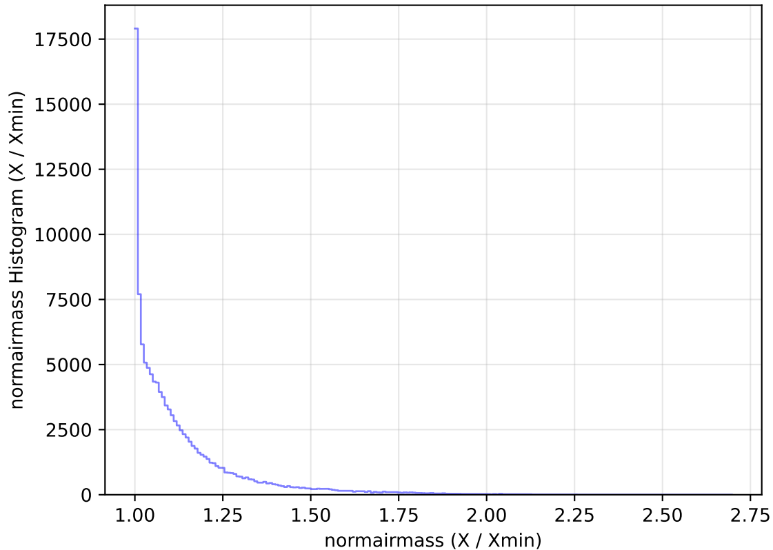
too_elab_heavy_r128_d2_ugrizy_v3.4_10yrs WFD u band: normairmass Histogram
