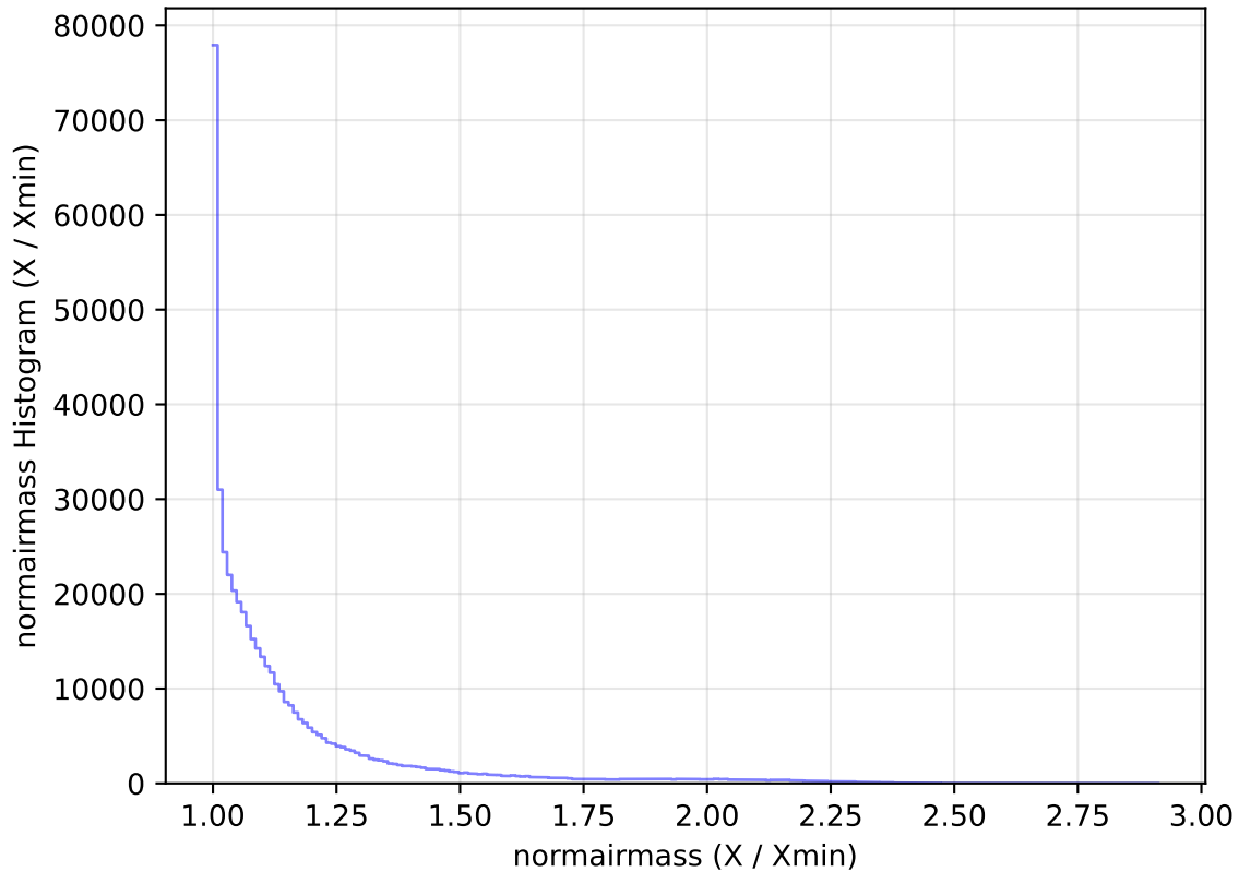
too_elab_heavy_r128_d2_ugrizy_v3.4_10yrs WFD r band: normairmass Histogram
