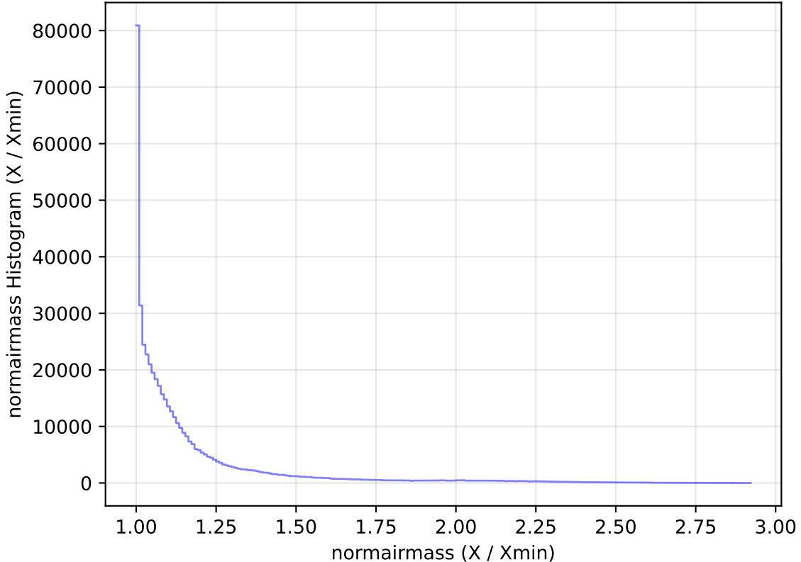
too_elab_heavy_r128_d2_ugrizy_v3.4_10yrs WFD i band: normairmass Histogram
