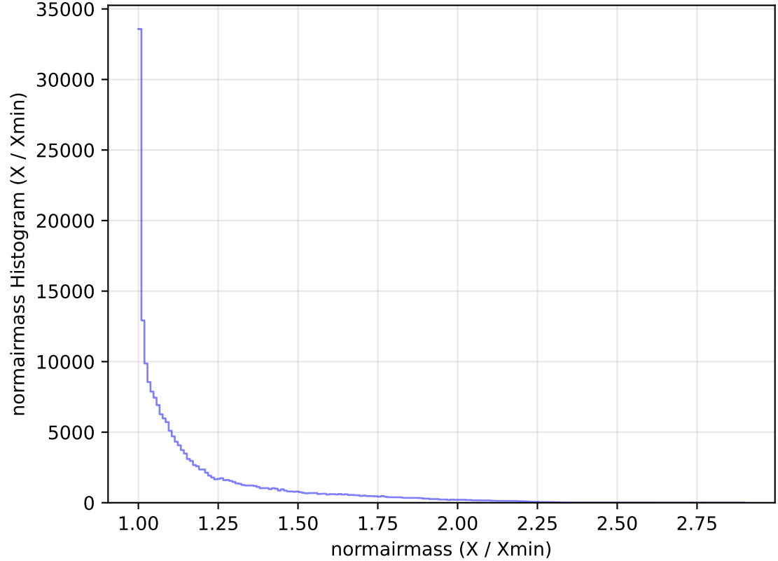
too_elab_heavy_r128_d2_ugrizy_v3.4_10yrs WFD g band: normairmass Histogram
