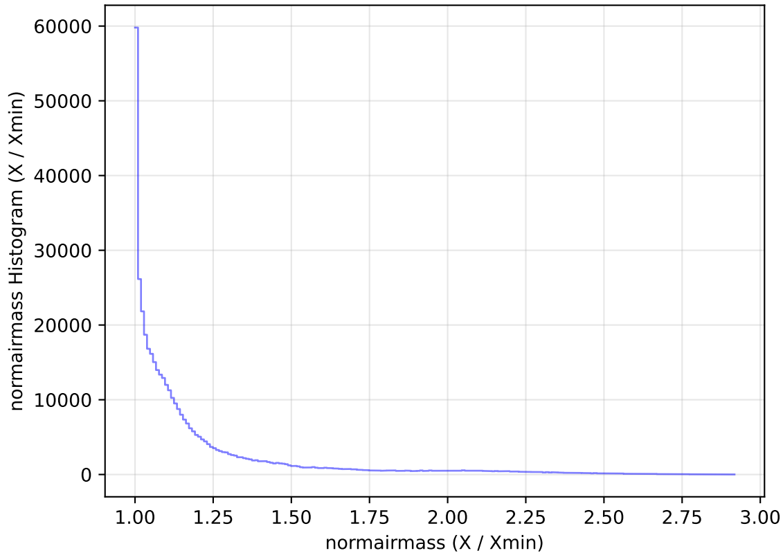
too_elab_heavy_r128_d2_ugrizy_v3.4_10yrs All sky z band: normairmass Histogram
