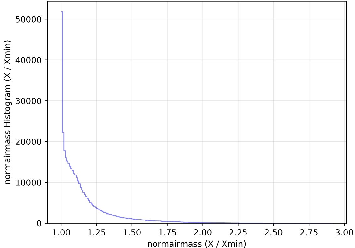
too_elab_heavy_r128_d2_ugrizy_v3.4_10yrs All sky y band: normairmass Histogram
