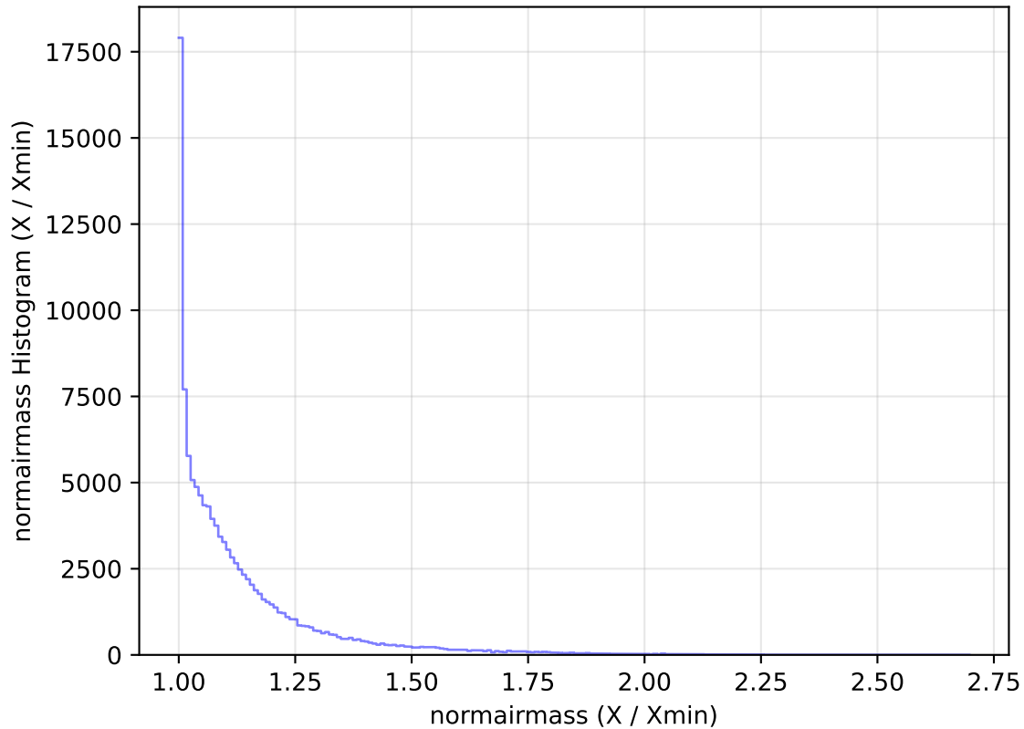
too_elab_heavy_r128_d2_ugrizy_v3.4_10yrs All sky u band: normairmass Histogram
