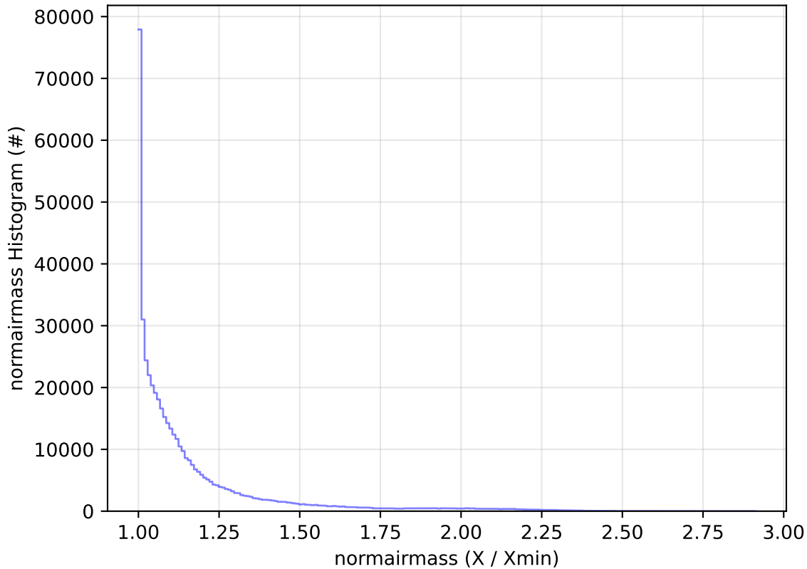
too_elab_heavy_r128_d2_ugrizy_v3.4_10yrs All sky r band: normairmass Histogram
