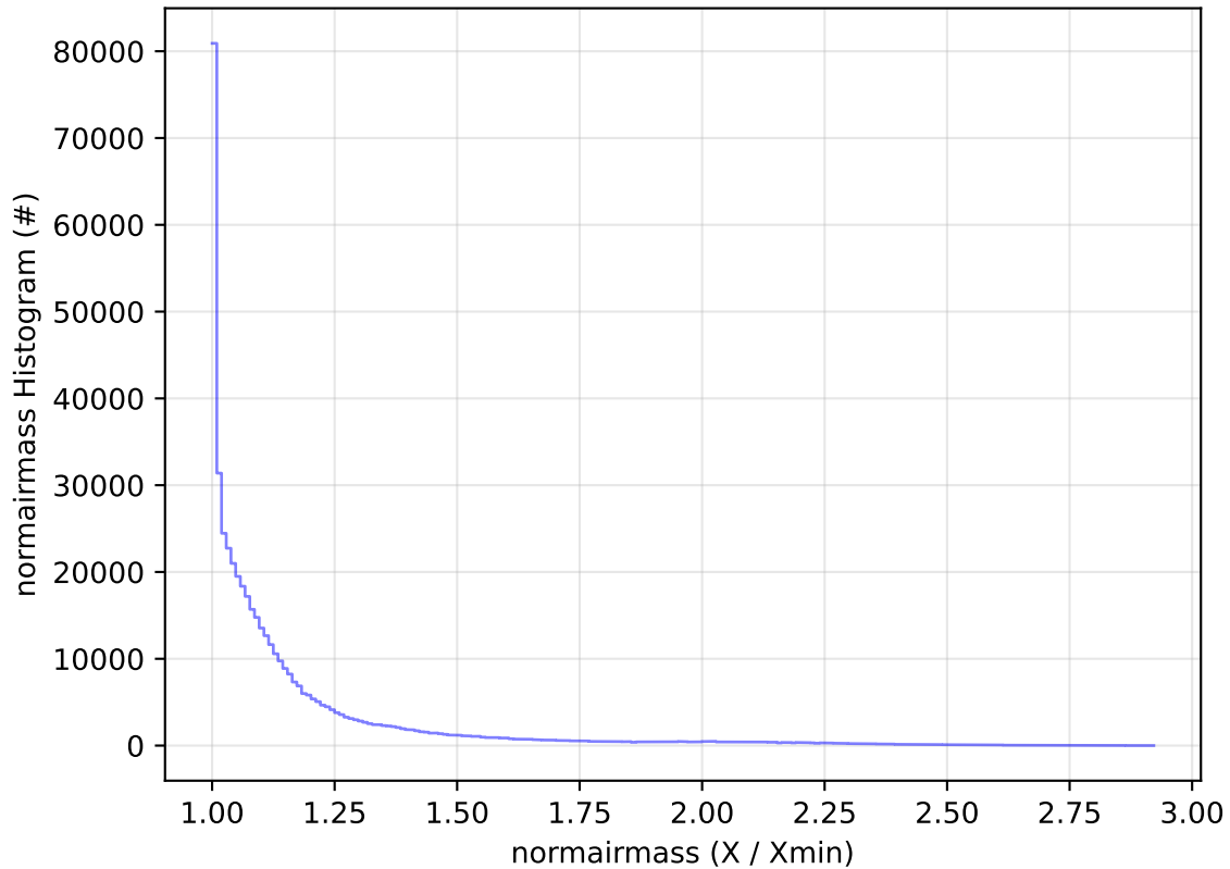
too_elab_heavy_r128_d2_ugrizy_v3.4_10yrs All sky i band: normairmass Histogram
