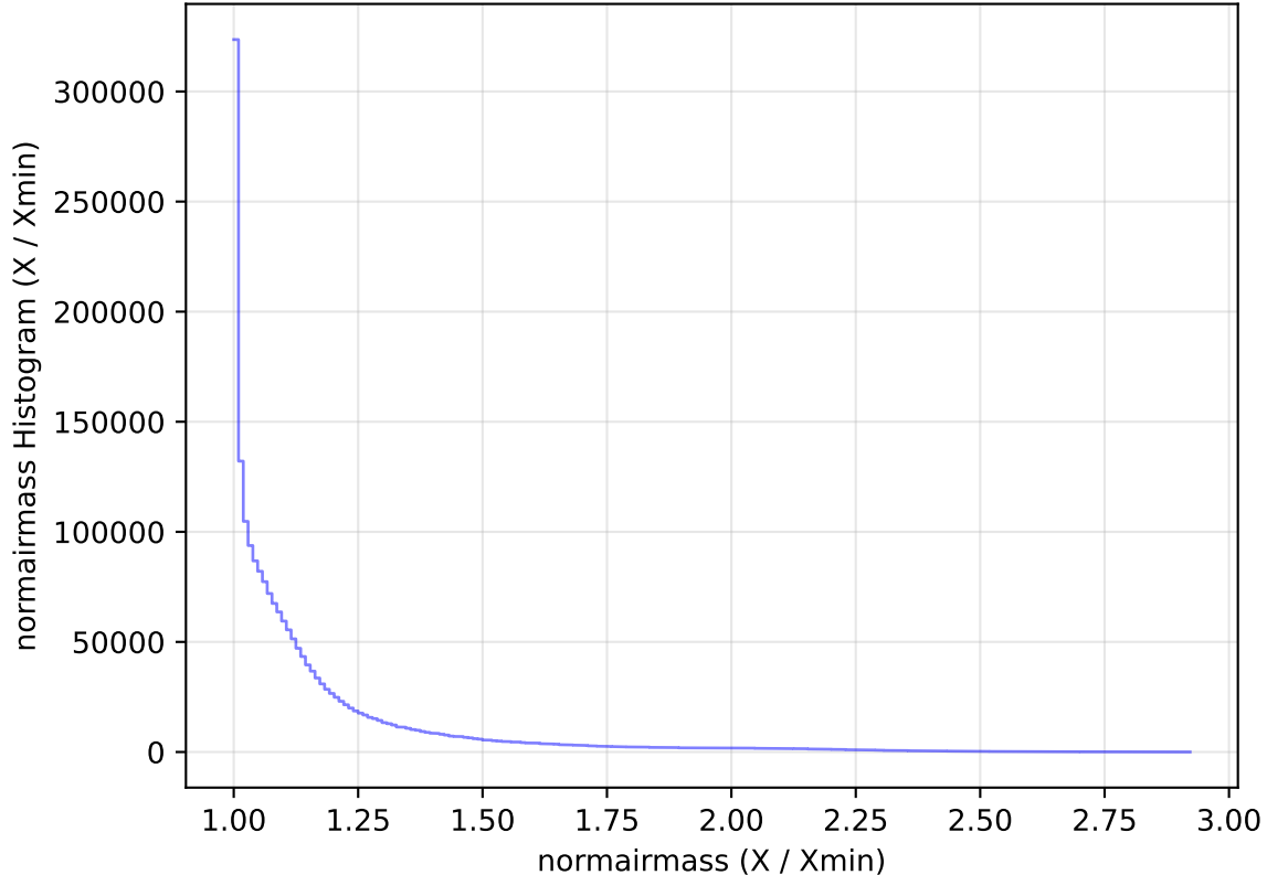
too_elab_heavy_r128_d2_ugrizy_v3.4_10yrs All sky all bands: normairmass Histogram
