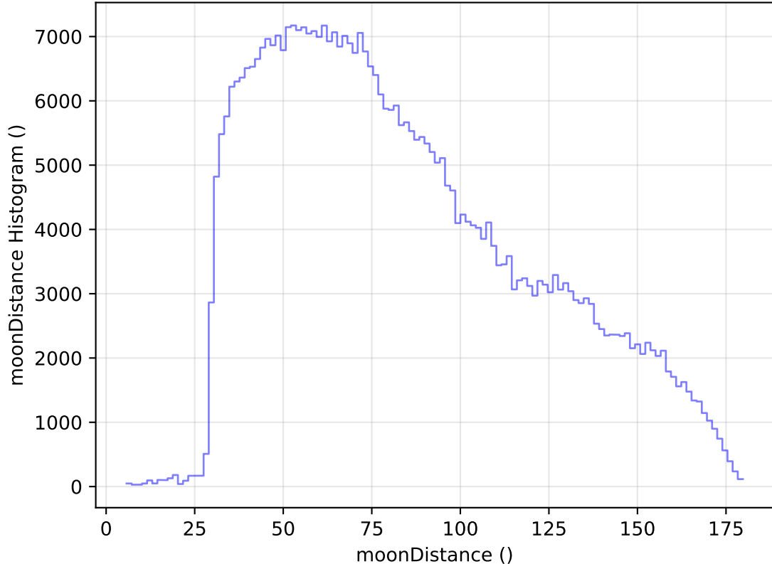
too_elab_heavy_r128_d2_ugrizy_v3.4_10yrs WFD z band: moonDistance Histogram
