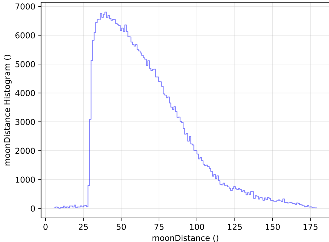
too_elab_heavy_r128_d2_ugrizy_v3.4_10yrs WFD y band: moonDistance Histogram
