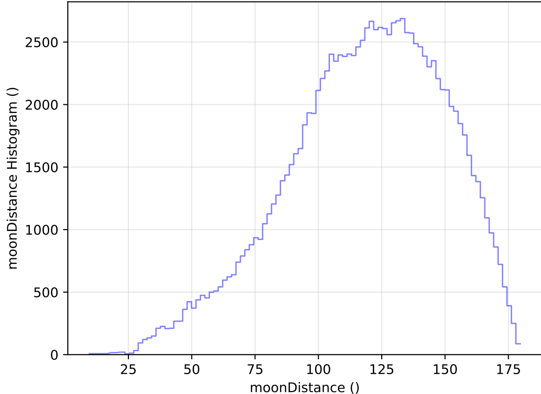
too_elab_heavy_r128_d2_ugrizy_v3.4_10yrs WFD u band: moonDistance Histogram
