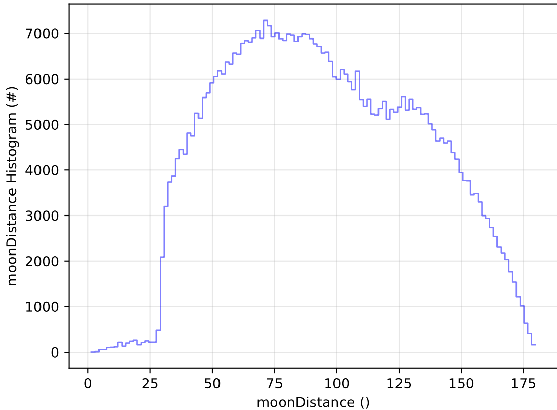
too_elab_heavy_r128_d2_ugrizy_v3.4_10yrs WFD i band: moonDistance Histogram
