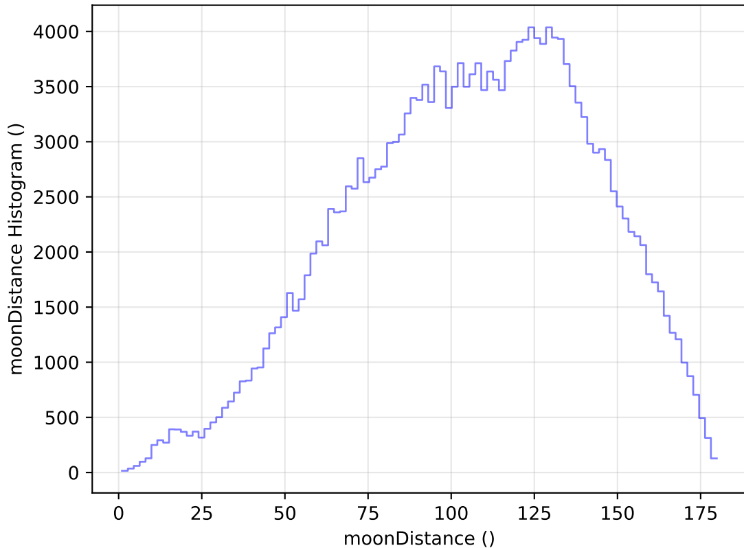
too_elab_heavy_r128_d2_ugrizy_v3.4_10yrs WFD g band: moonDistance Histogram
