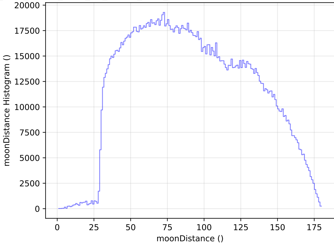
too_elab_heavy_r128_d2_ugrizy_v3.4_10yrs WFD all bands: moonDistance Histogram
