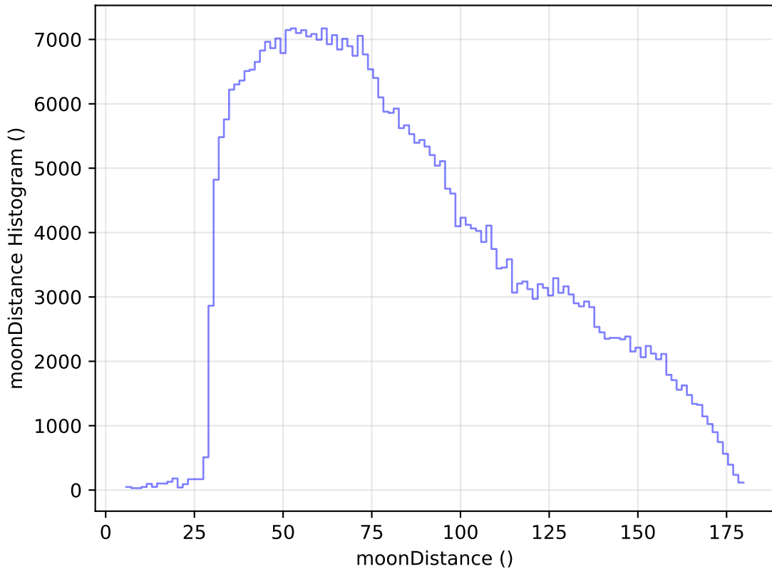
too_elab_heavy_r128_d2_ugrizy_v3.4_10yrs All sky z band: moonDistance Histogram
