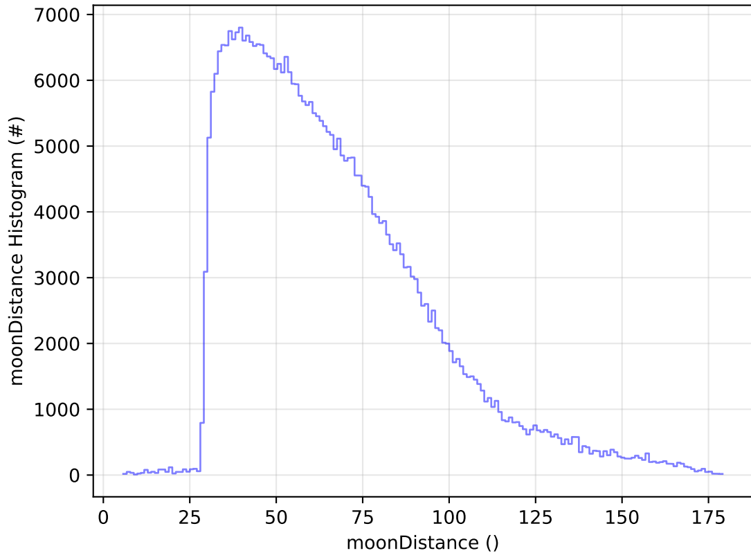
too_elab_heavy_r128_d2_ugrizy_v3.4_10yrs All sky y band: moonDistance Histogram
