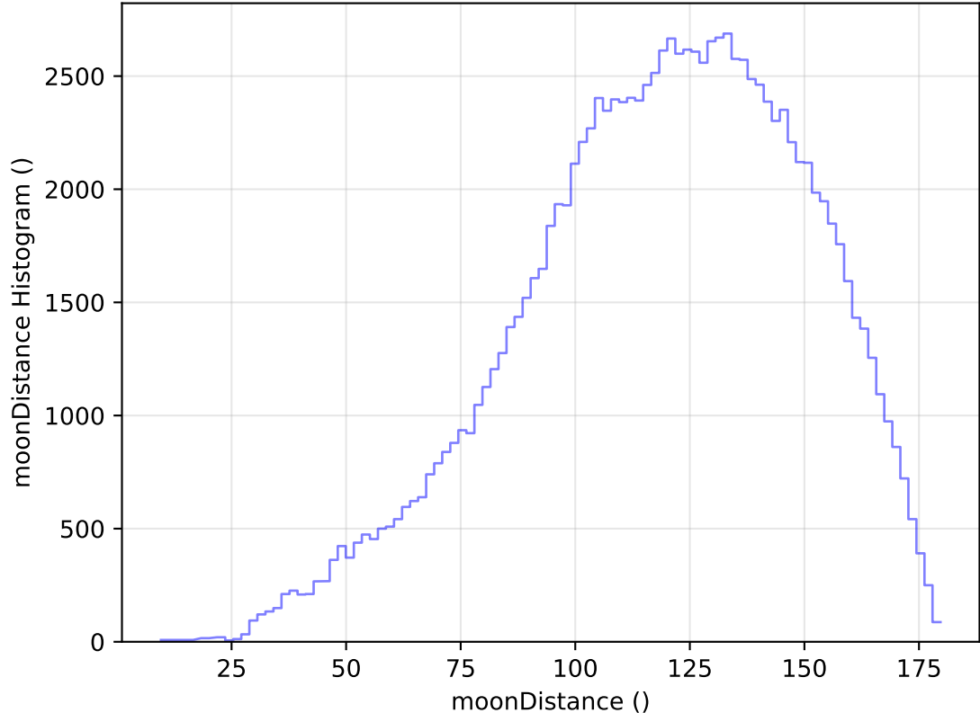
too_elab_heavy_r128_d2_ugrizy_v3.4_10yrs All sky u band: moonDistance Histogram
