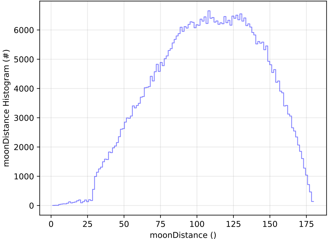
too_elab_heavy_r128_d2_ugrizy_v3.4_10yrs All sky r band: moonDistance Histogram
