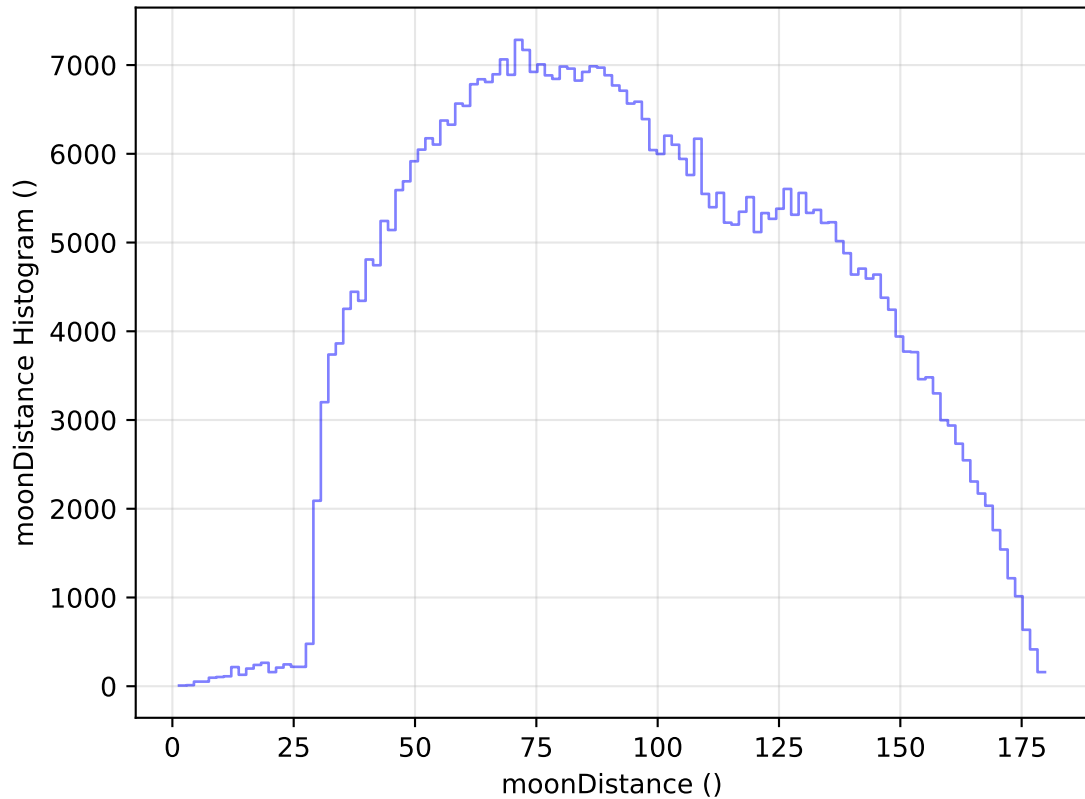
too_elab_heavy_r128_d2_ugrizy_v3.4_10yrs All sky i band: moonDistance Histogram
