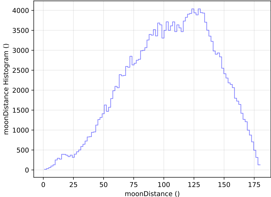
too_elab_heavy_r128_d2_ugrizy_v3.4_10yrs All sky g band: moonDistance Histogram
