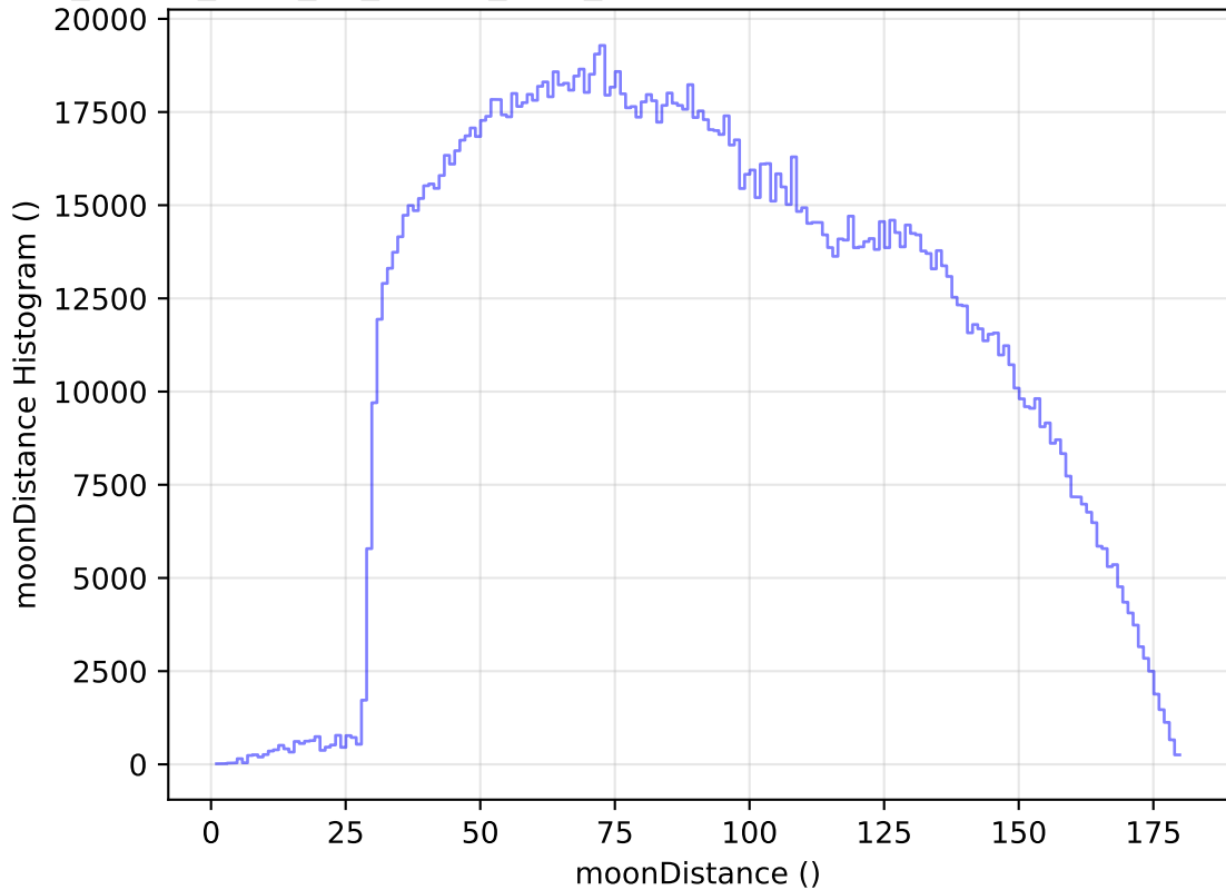
too_elab_heavy_r128_d2_ugrizy_v3.4_10yrs All sky all bands: moonDistance Histogram
