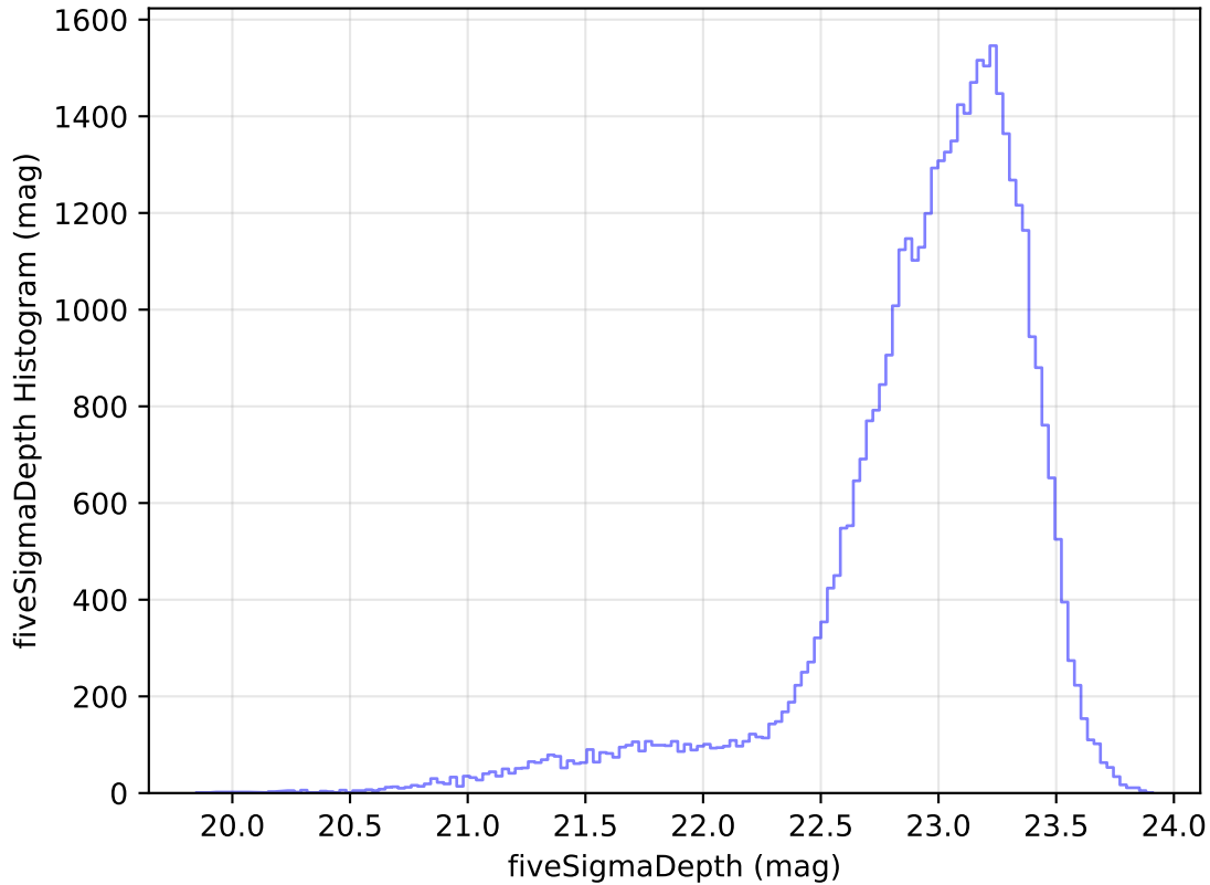
too_elab_heavy_r128_d2_ugrizy_v3.4_10yrs Yr 1 z band: fiveSigmaDepth Histogram
