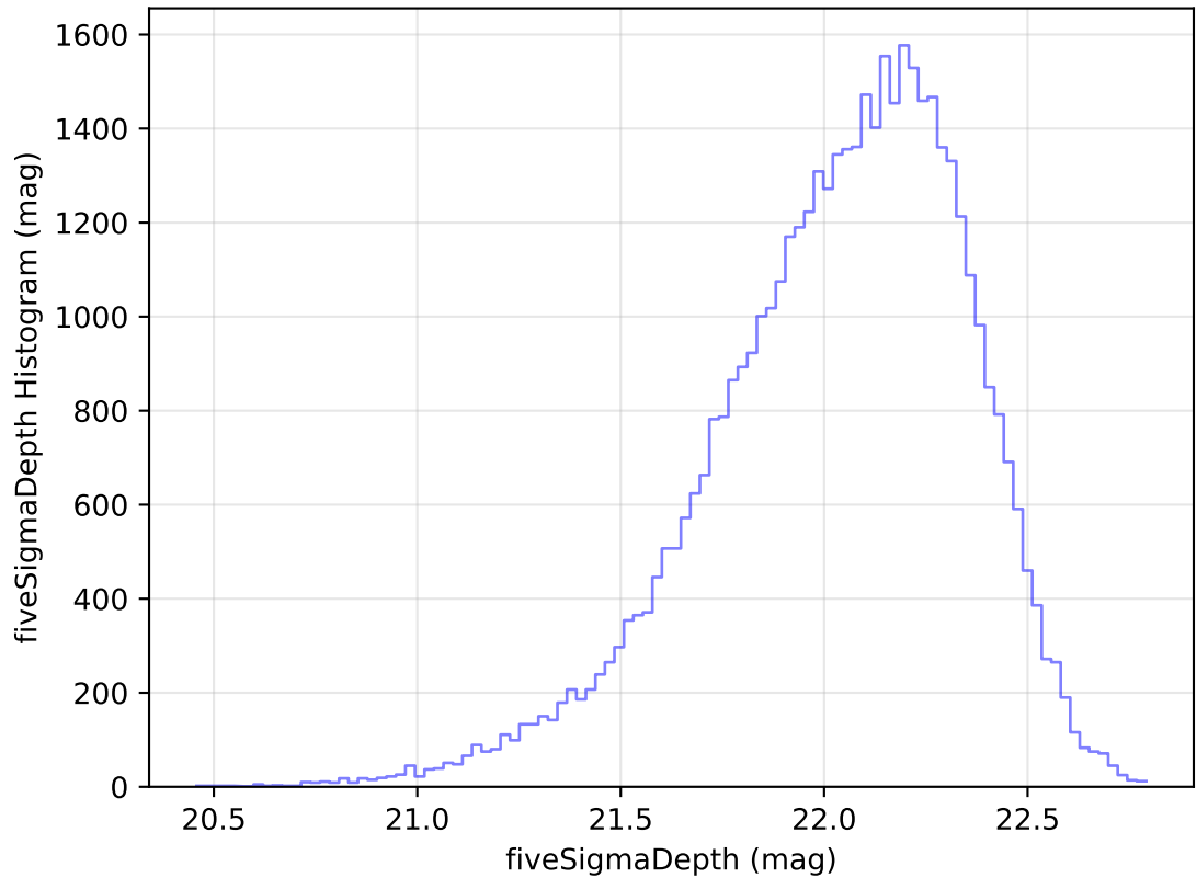
too_elab_heavy_r128_d2_ugrizy_v3.4_10yrs Yr 1 y band: fiveSigmaDepth Histogram
