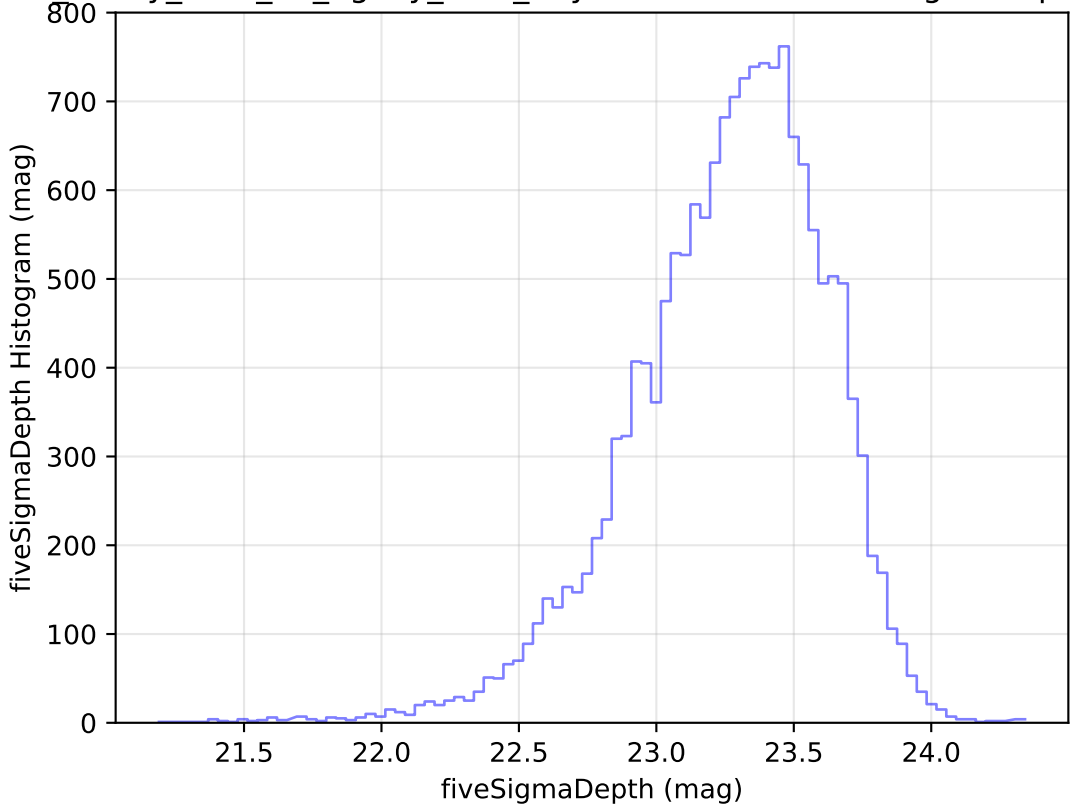
too_elab_heavy_r128_d2_ugrizy_v3.4_10yrs Yr 1 u band: fiveSigmaDepth Histogram
