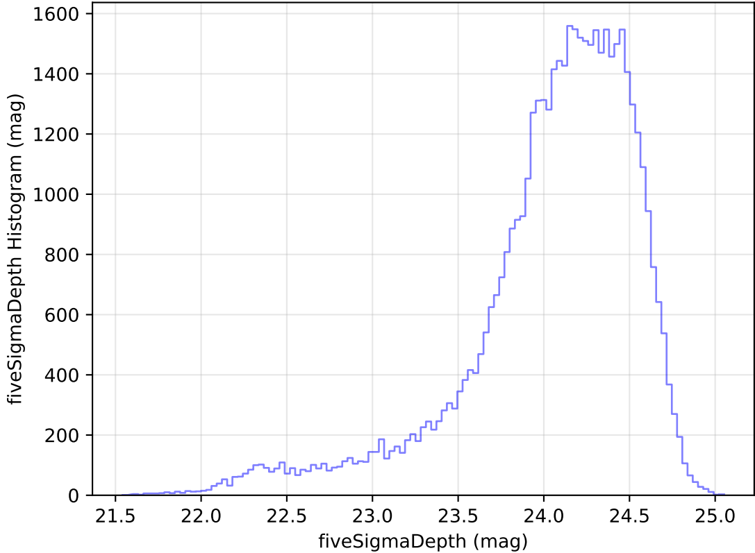
too_elab_heavy_r128_d2_ugrizy_v3.4_10yrs Yr 1 r band: fiveSigmaDepth Histogram
