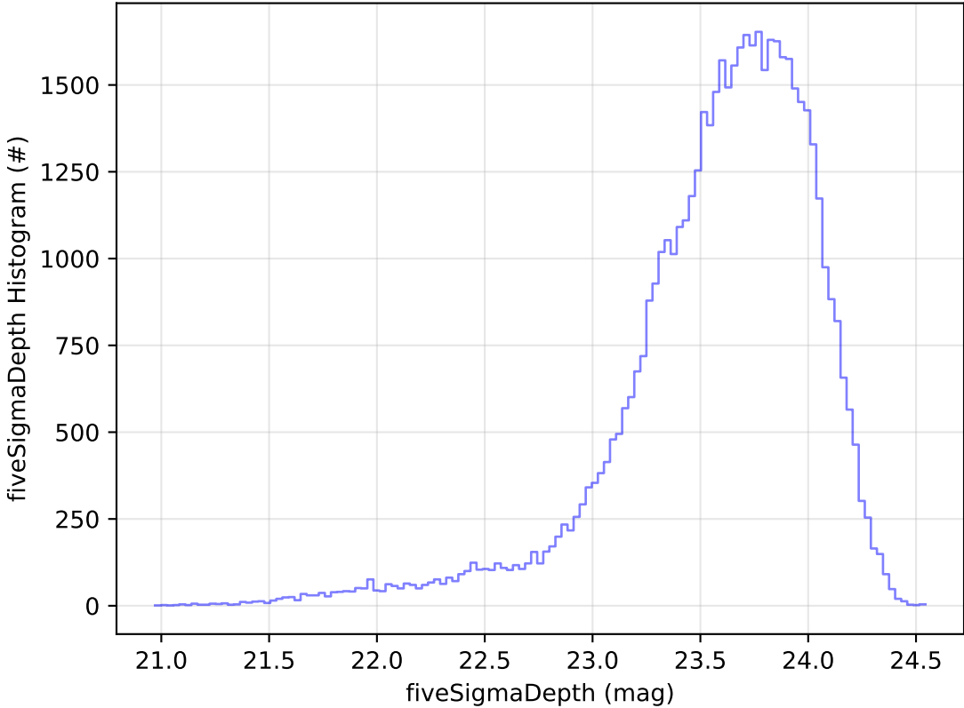
too_elab_heavy_r128_d2_ugrizy_v3.4_10yrs Yr 1 i band: fiveSigmaDepth Histogram
