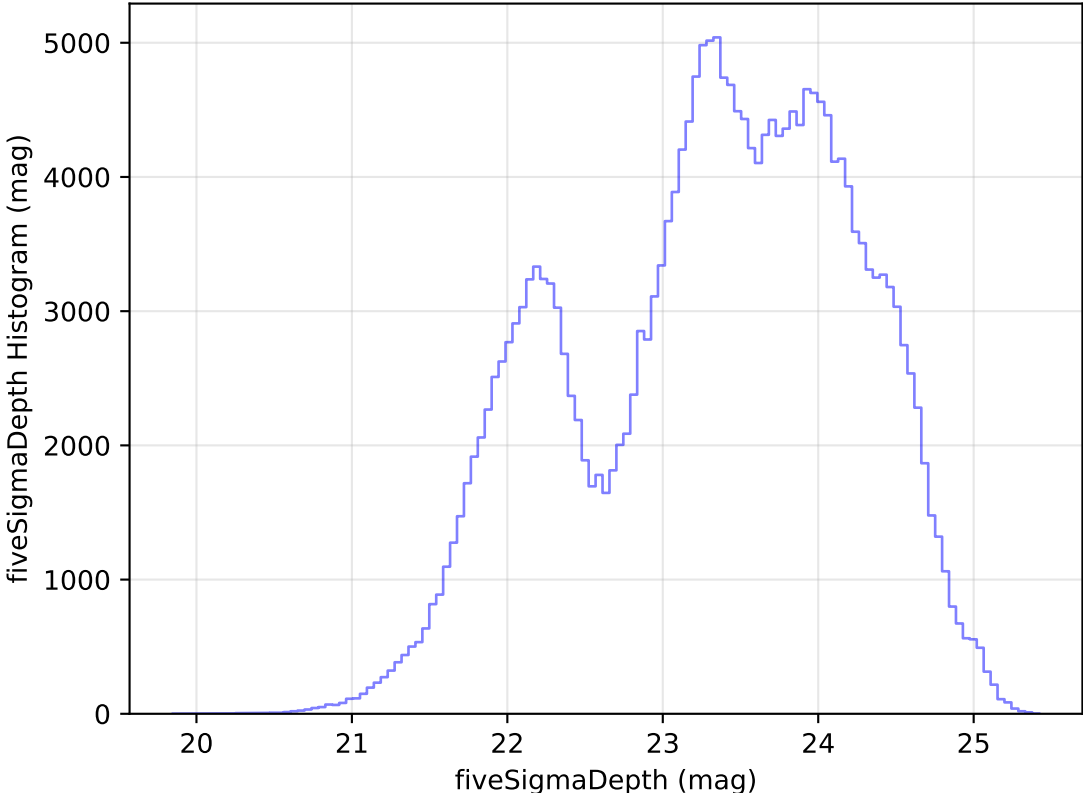
too_elab_heavy_r128_d2_ugrizy_v3.4_10yrs Yr 1 all bands: fiveSigmaDepth Histogram
