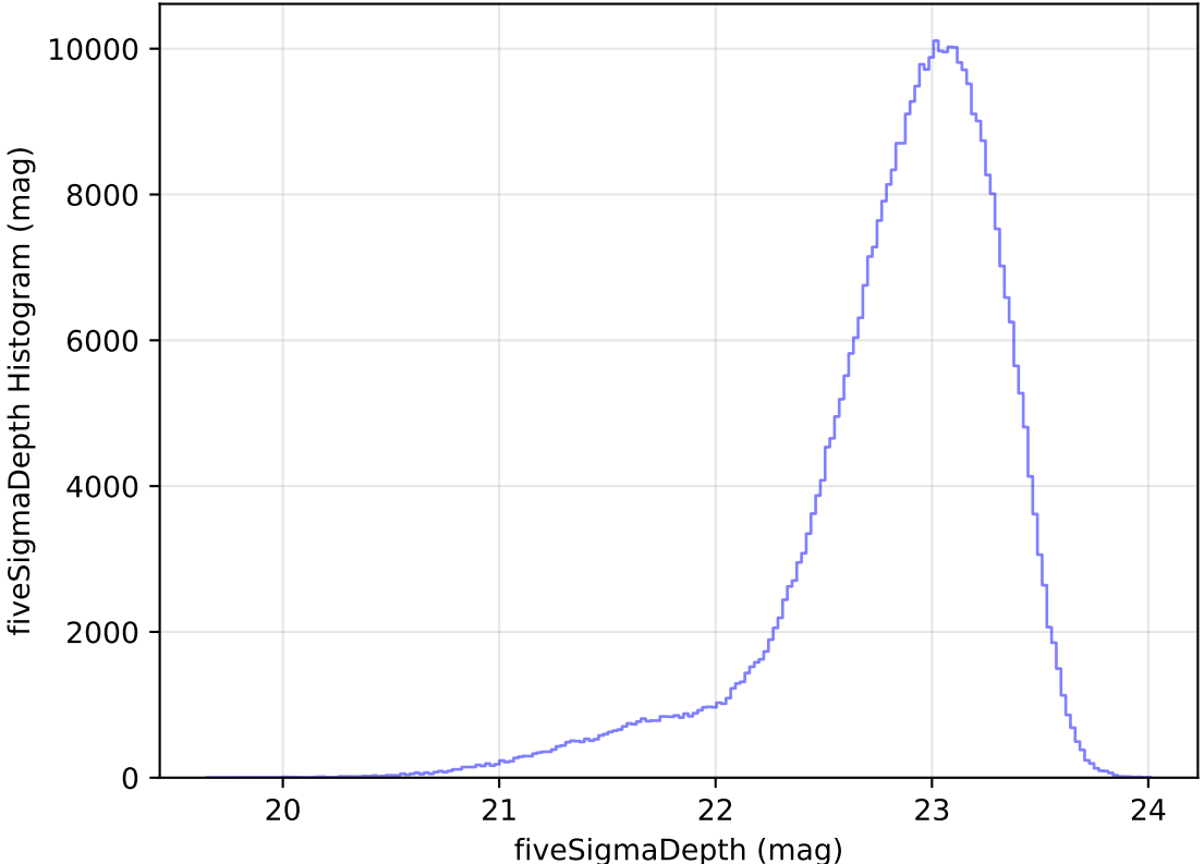
too_elab_heavy_r128_d2_ugrizy_v3.4_10yrs WFD z band: fiveSigmaDepth Histogram
