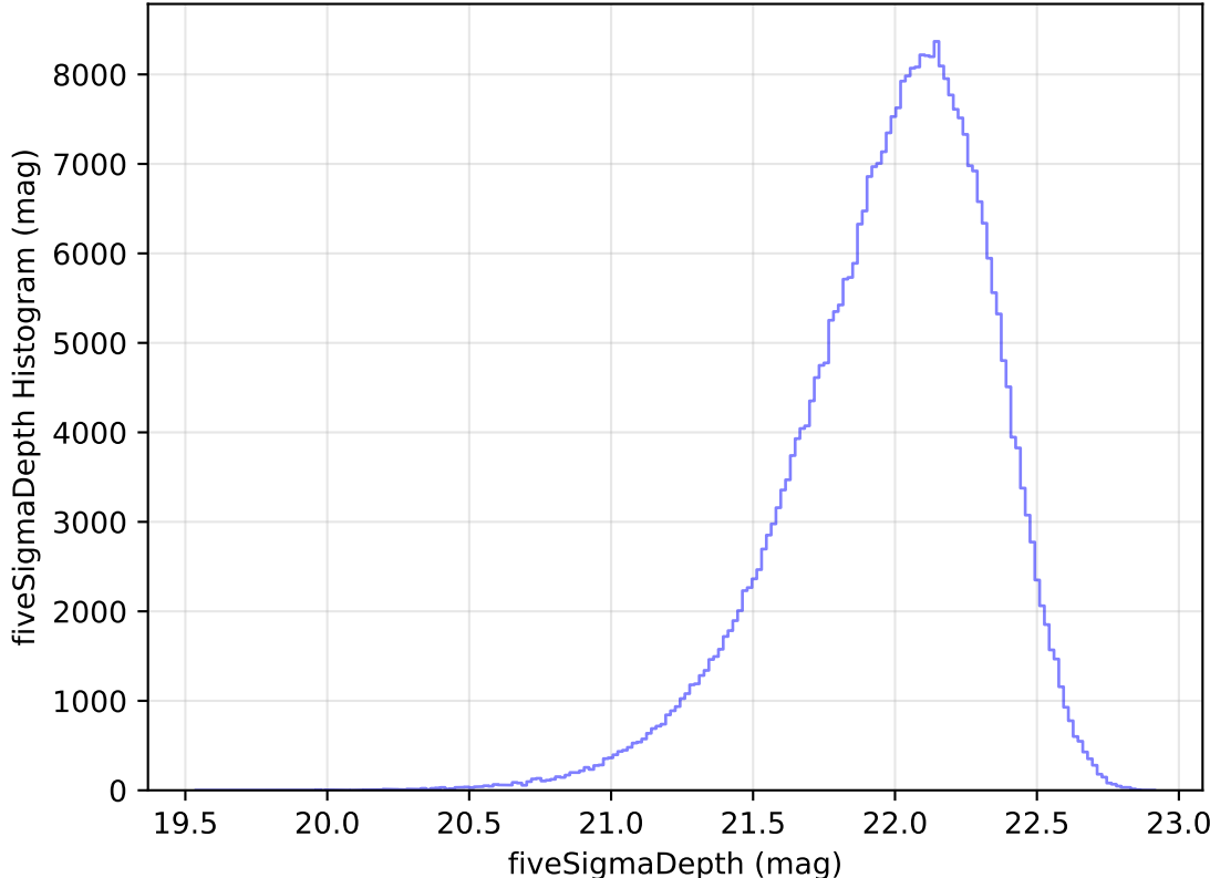
too_elab_heavy_r128_d2_ugrizy_v3.4_10yrs WFD y band: fiveSigmaDepth Histogram
