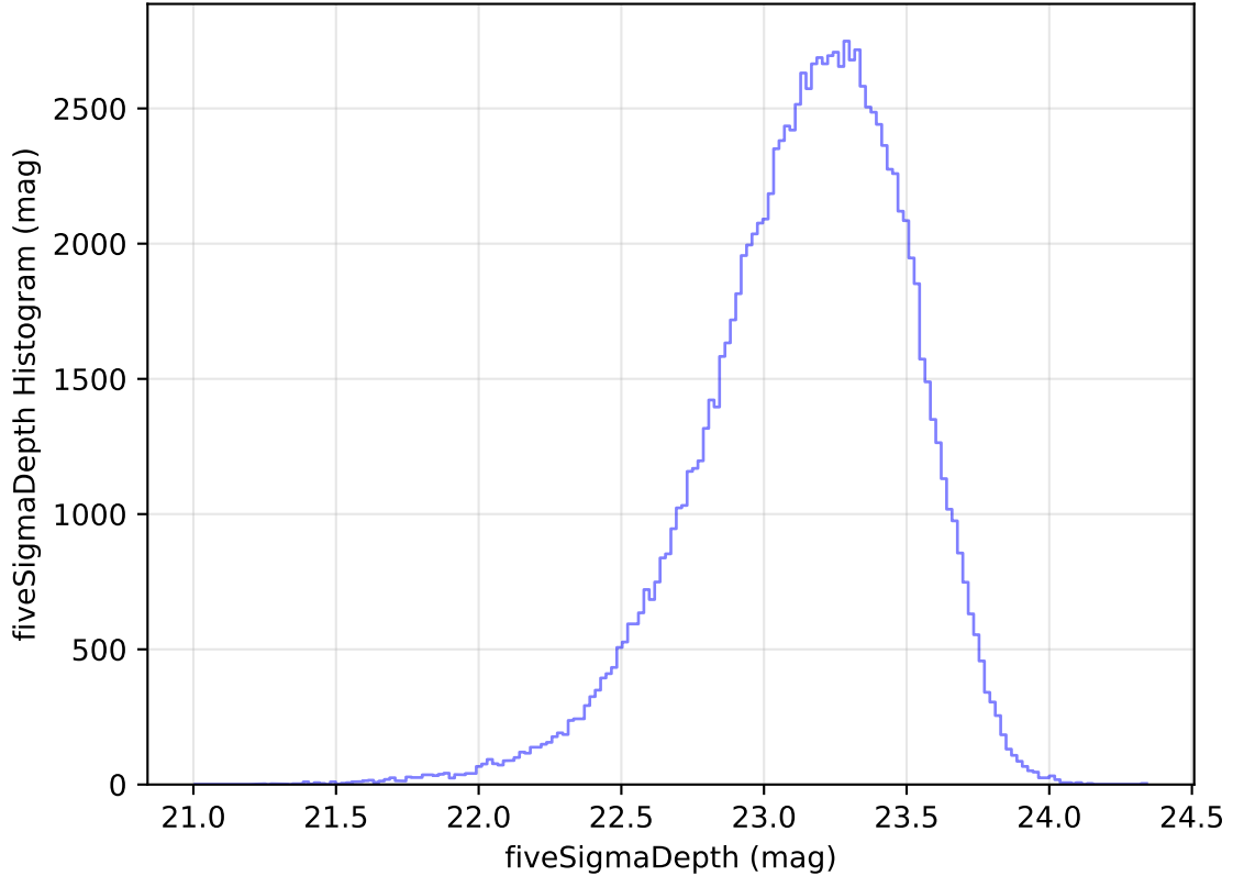
too_elab_heavy_r128_d2_ugrizy_v3.4_10yrs WFD u band: fiveSigmaDepth Histogram
